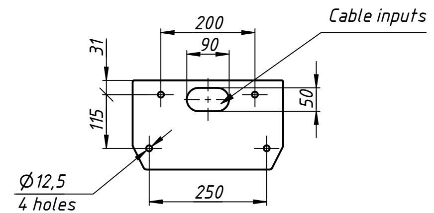
Installation tamplate
