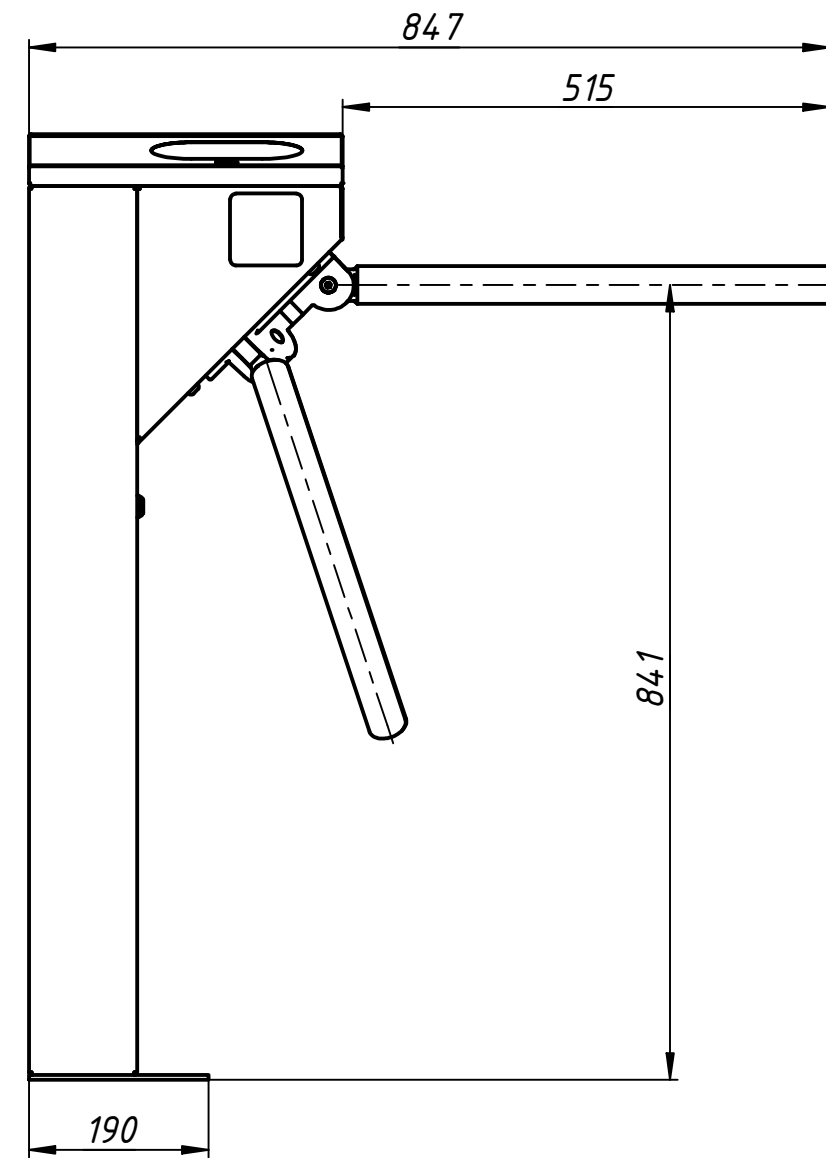
Installation tamplate
